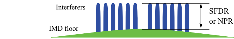
FIGURE 18 Spurious-free dynamic range or noise power ratio of a multichannel system.
