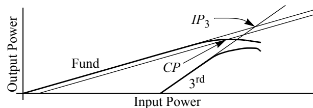
FIGURE 15 The 1 dB compression point ( CP_1 ) is the point where the output power of the fundamental crosses the line that represents the output power extrapolated from small-signal conditions minus 1 dB. The 3 rd order intercept point ( IP_3 ) is the point where the third-order term as extrapolated from small-signal conditions crosses the extrapolated power of the fundamental.
