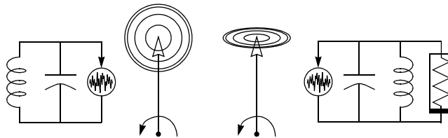
FIGURE 8 A linear oscillator along with its response to noise (left) and a nonlinear oscillator with its response to noise (right). The arrows are phasors that represents the unperturbed oscillator output, the carriers, and the circles represent the response to perturbations in the form of noise. With a linear oscillator the noise simply adds to the carrier. In a nonlinear oscillator, the nonlinearities act to control the amplitude of the oscillator and so to suppress variations in amplitude, thereby radially compressing the noise ball and converting it into predominantly a variation in phase.
